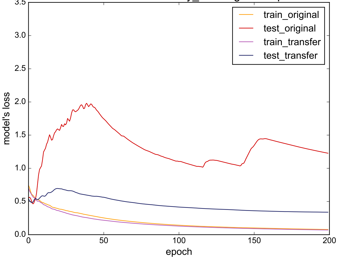
Source: uWaveGestureLibrary_Z - Target: ShapeletSim
