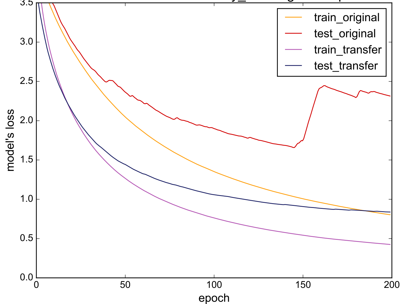
Source: uWaveGestureLibrary_Z - Target: ShapesAll
