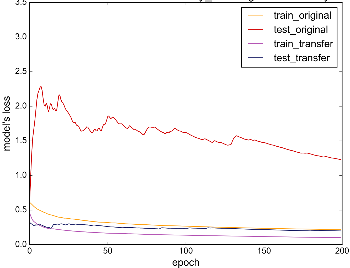
Source: uWaveGestureLibrary_Z - Target: Strawberry
