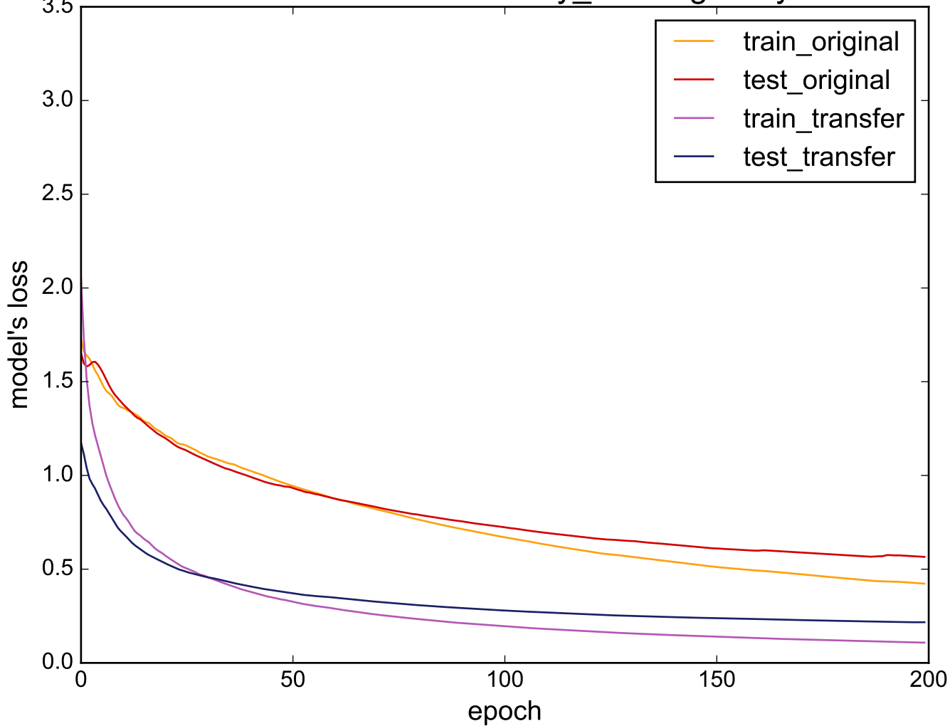
Source: uWaveGestureLibrary_Z - Target: Symbols
