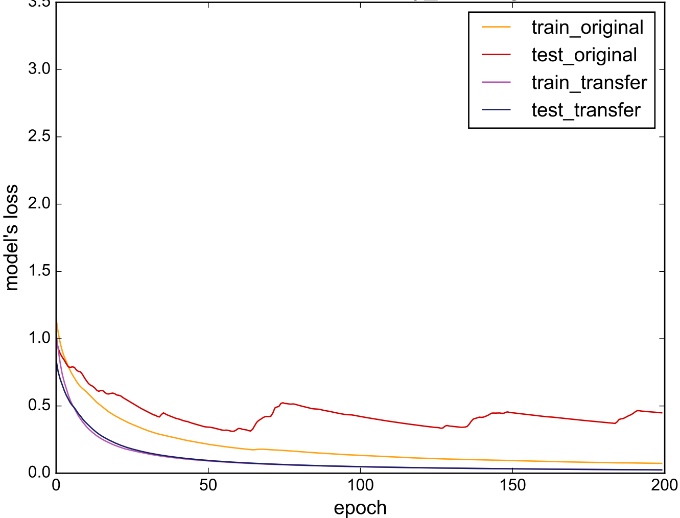
Source: uWaveGestureLibrary_Z - Target: Trace
