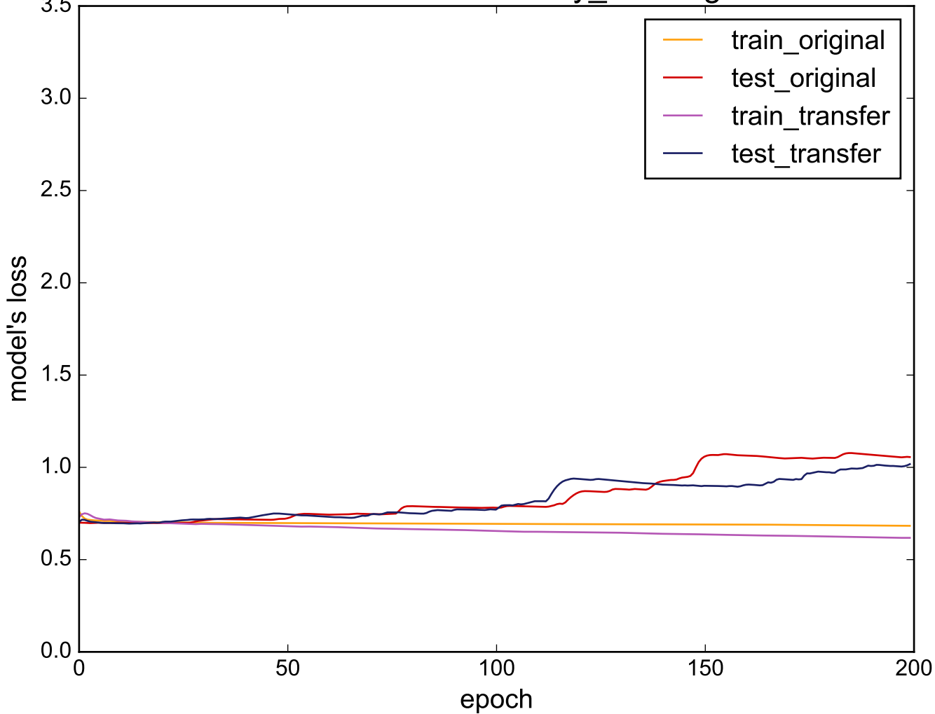
Source: uWaveGestureLibrary_Z - Target: Wine
