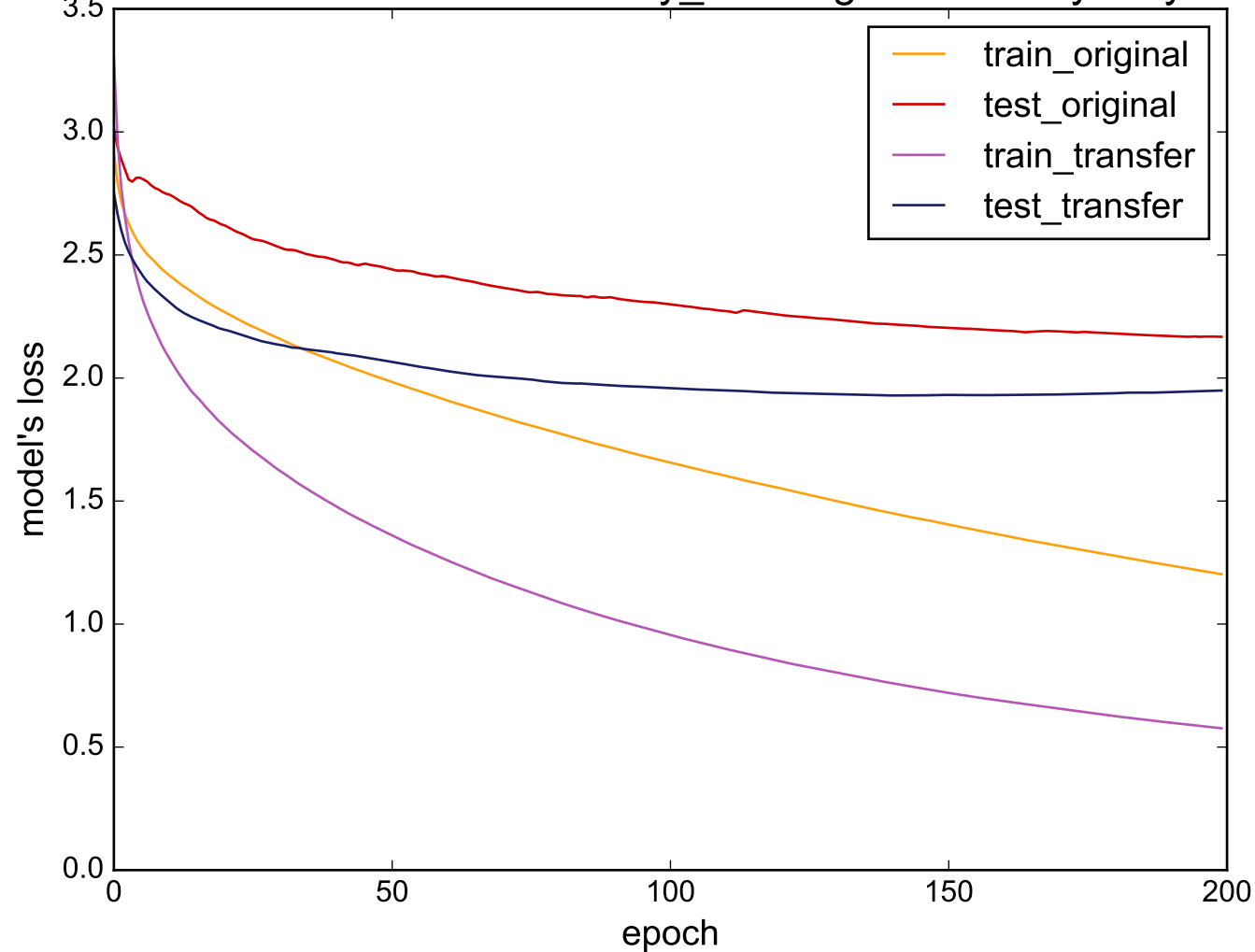
Source: uWaveGestureLibrary_Z - Target: WordsSynonyms
