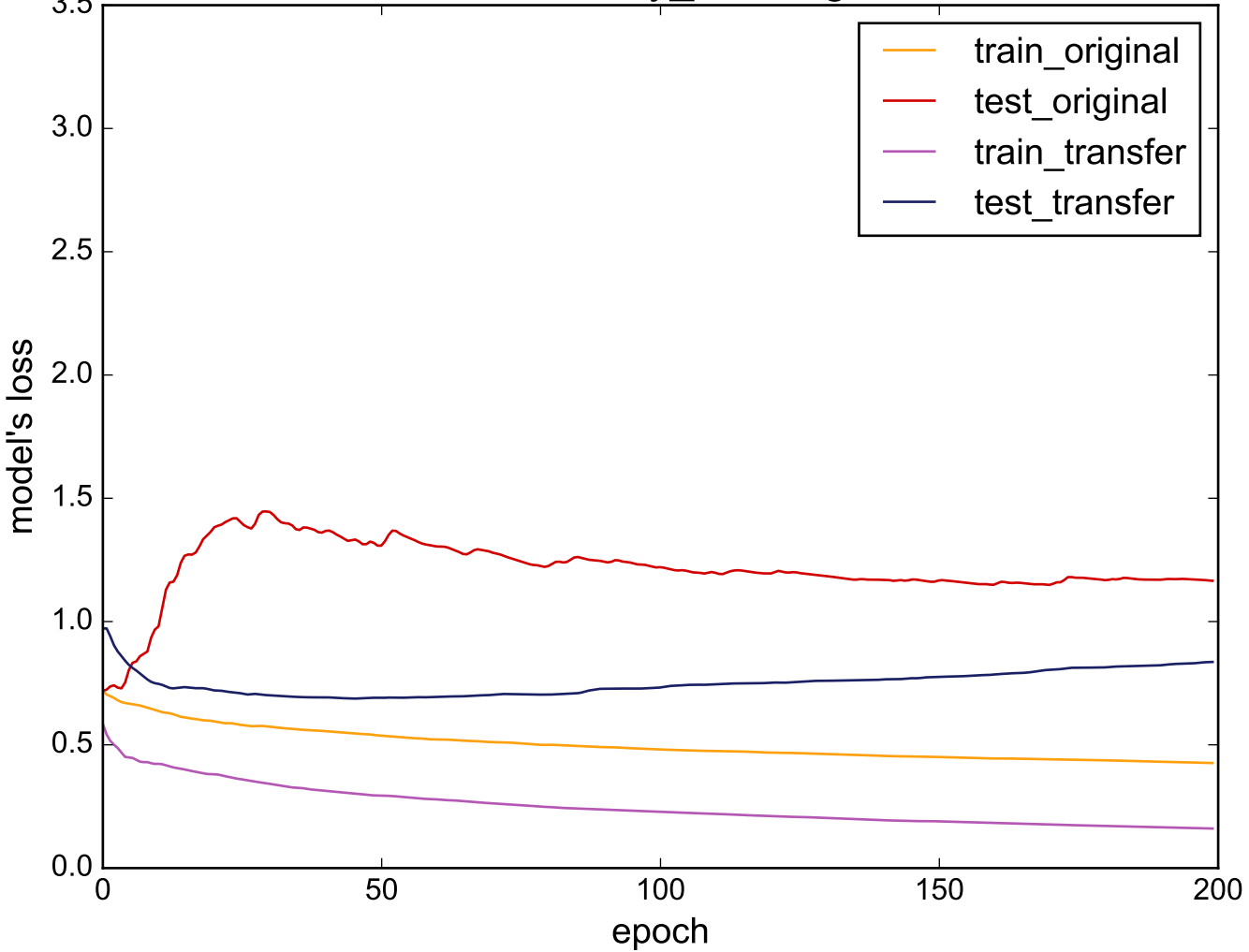
Source: uWaveGestureLibrary_Z - Target: WormsTwoClass
