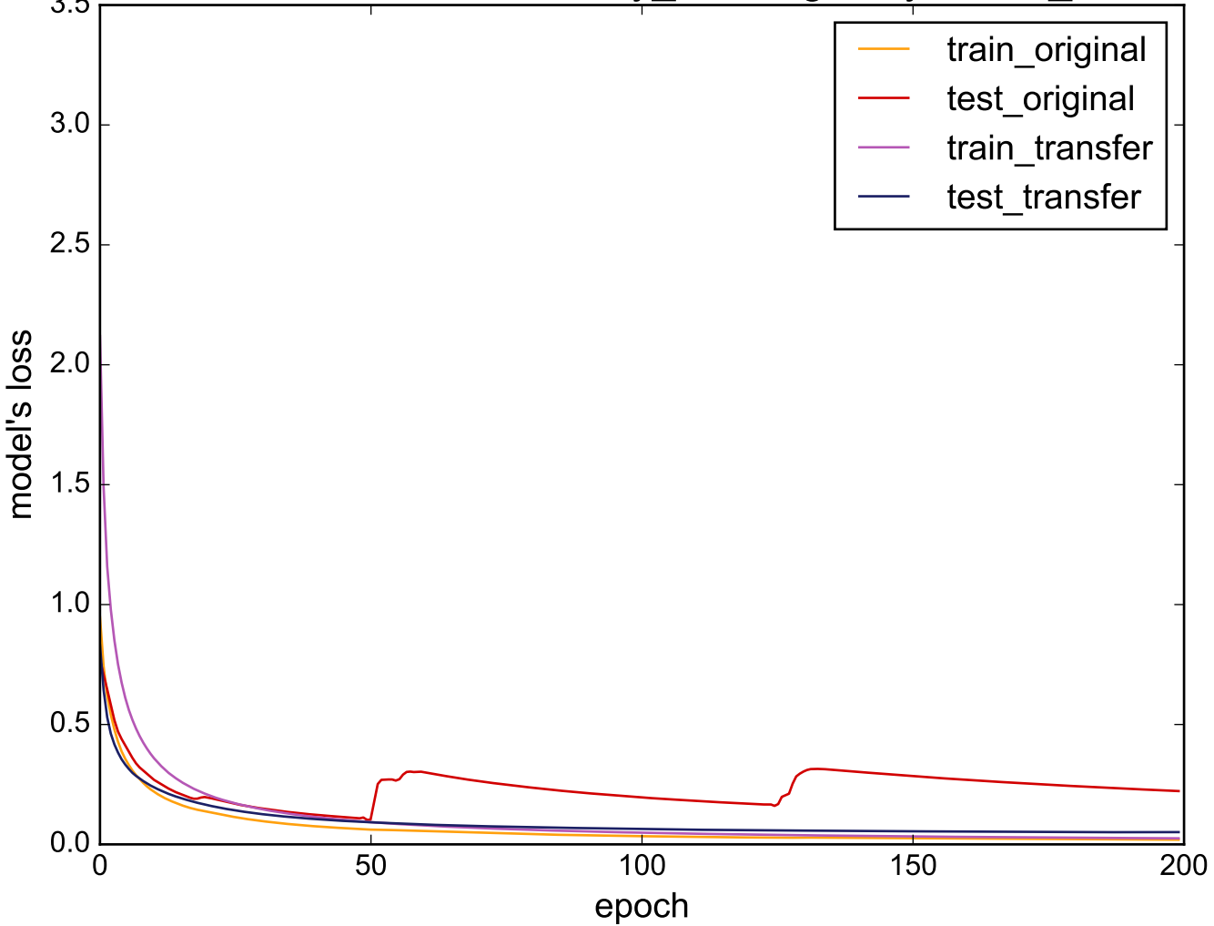
Source: uWaveGestureLibrary_Z - Target: synthetic_control
