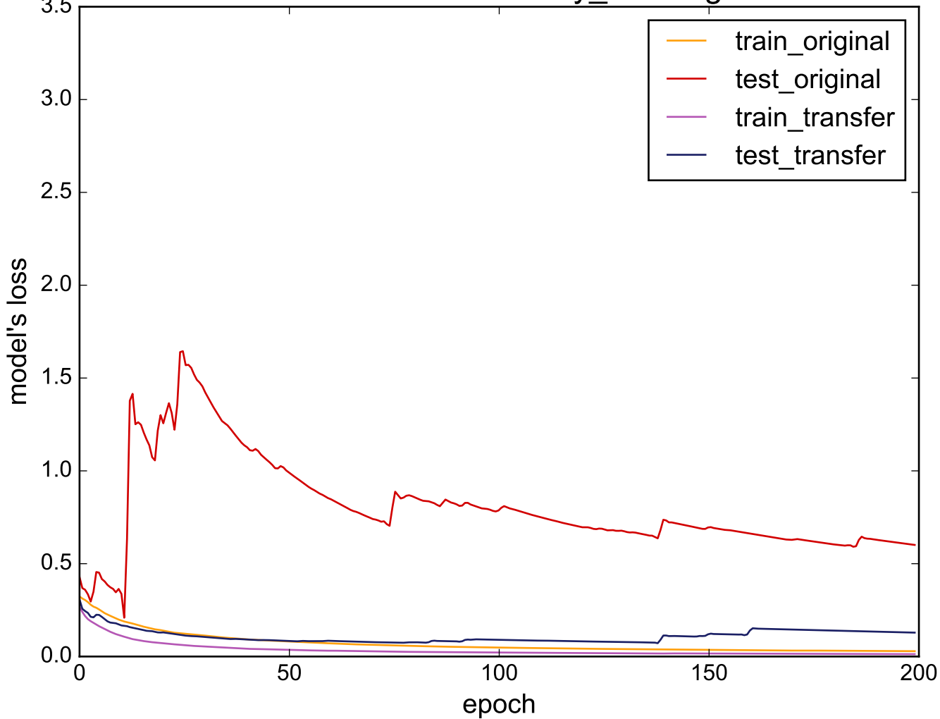
Source: uWaveGestureLibrary_Z - Target: wafer
