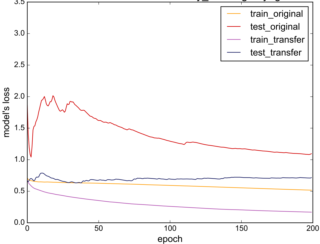
Source: uWaveGestureLibrary_Z - Target: yoga
