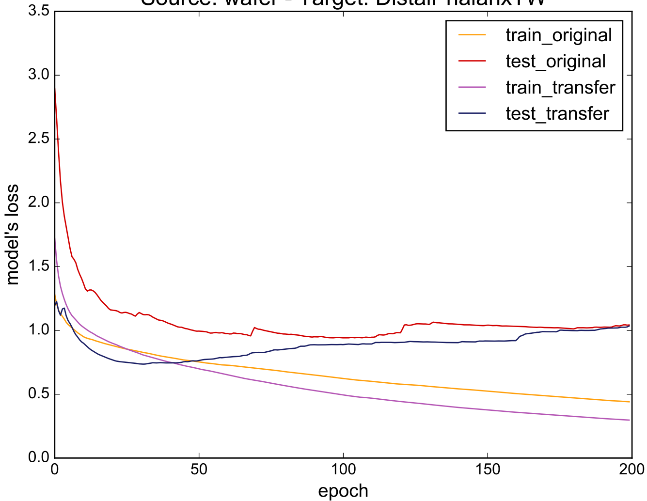
Source: wafer - Target: DistalPhalanxTW
