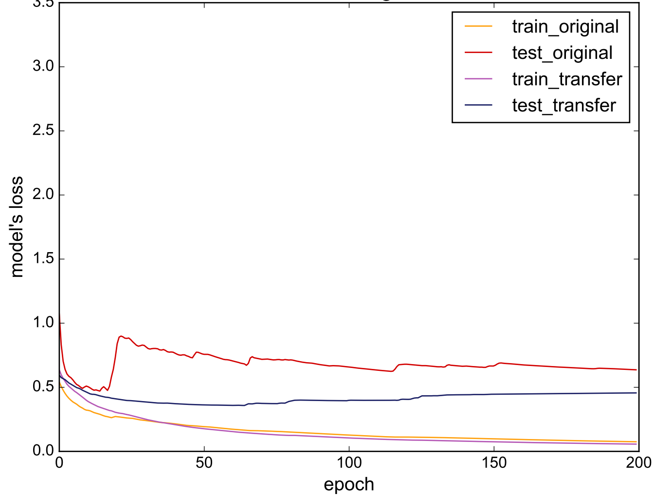
Source: wafer - Target: ECG200
