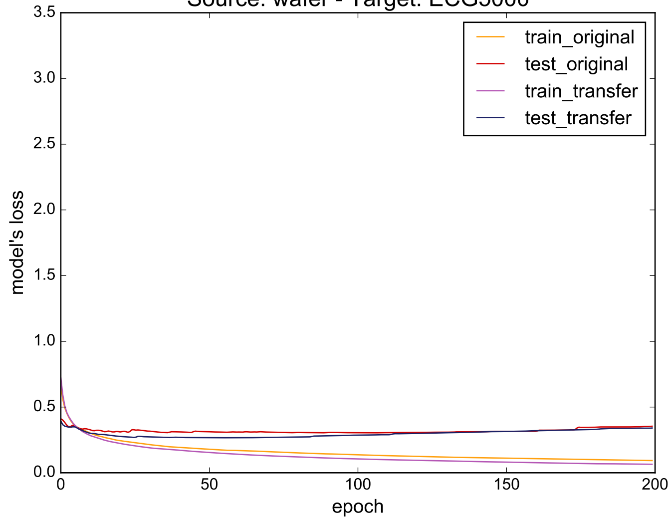
Source: wafer - Target: ECG5000
