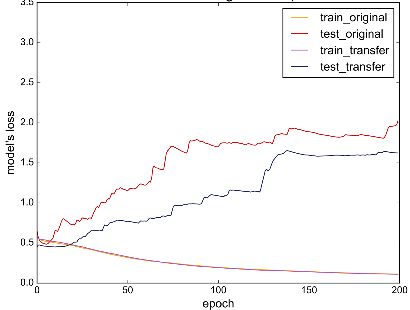
Source: wafer - Target: Earthquakes
