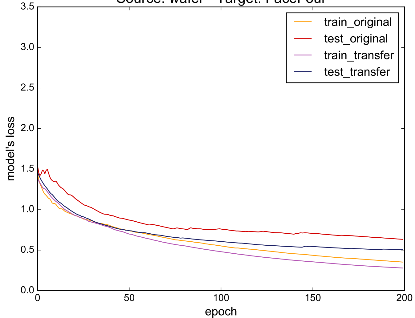
Source: wafer - Target: FaceFour
