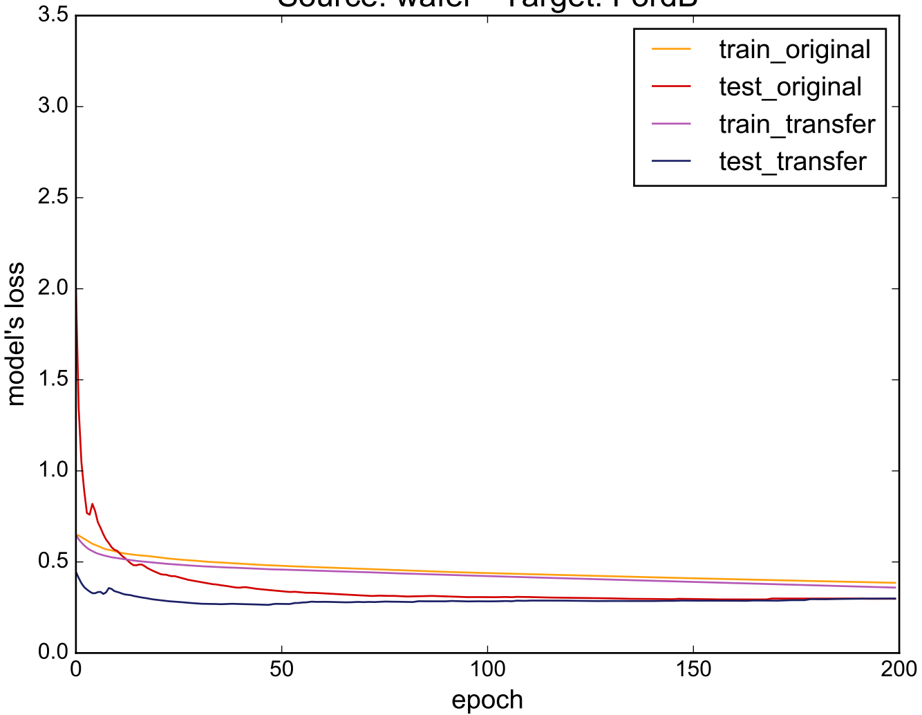
Source: wafer - Target: FordB
