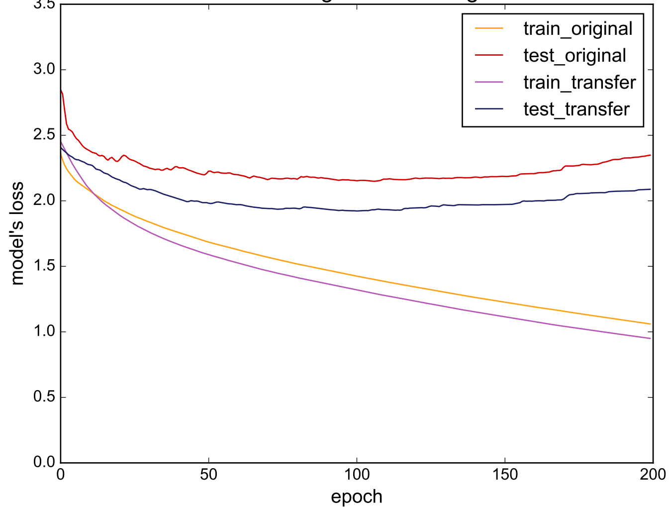
Source: wafer - Target: InsectWingbeatSound
