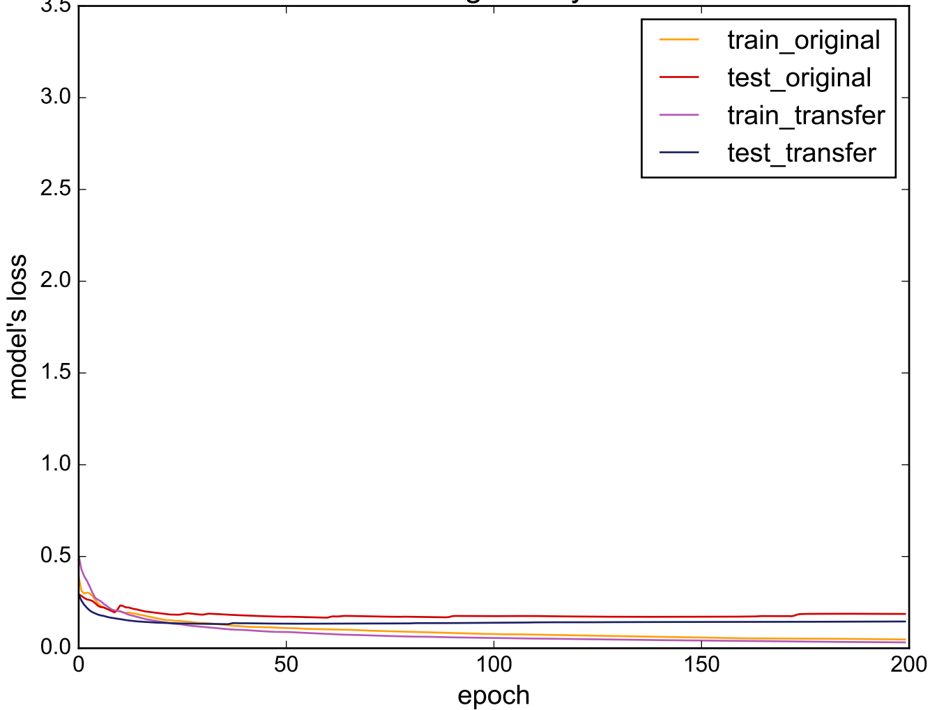
Source: wafer - Target: ItalyPowerDemand
