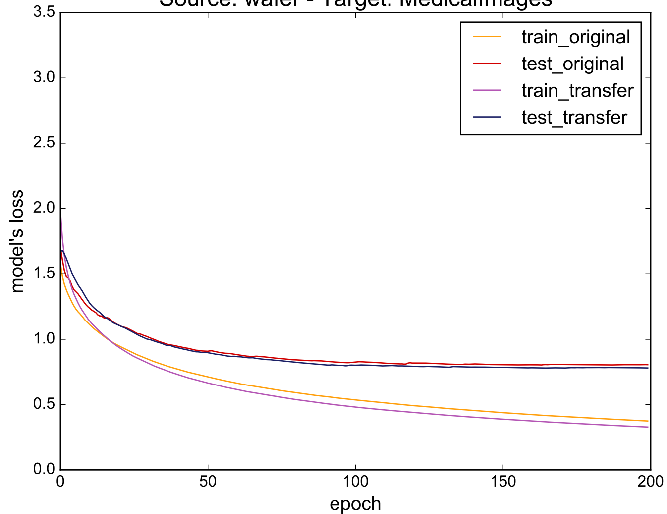
Source: wafer - Target: MedicalImages
