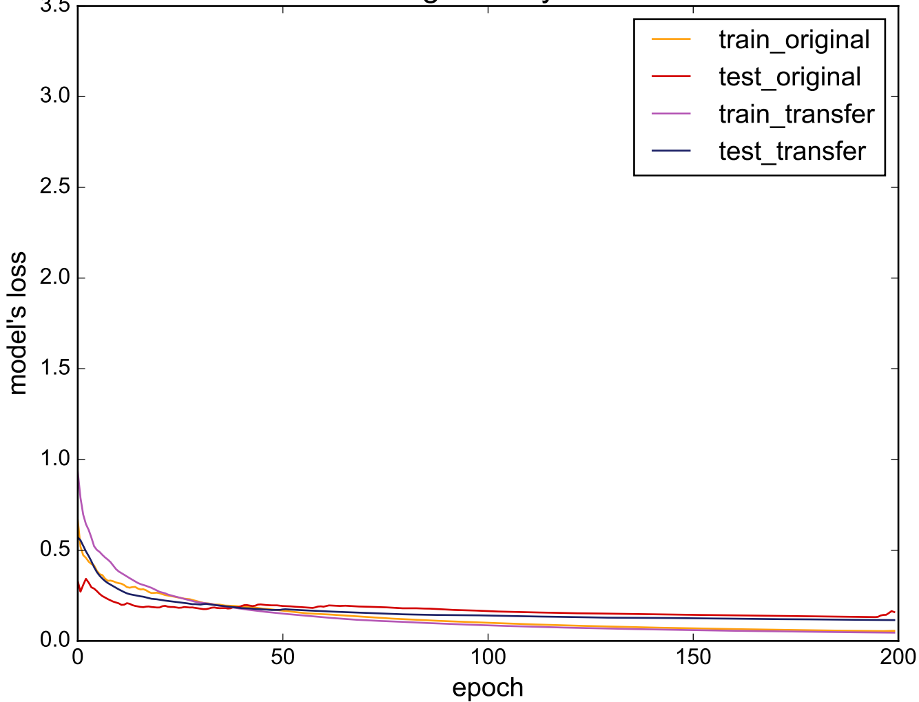
Source: wafer - Target: SonyAIBORobotSurface
