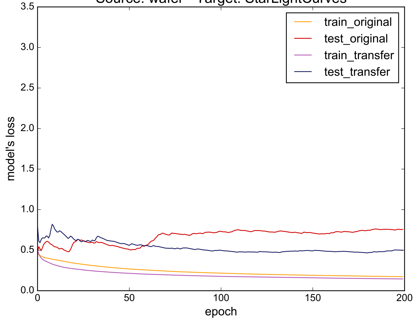
Source: wafer - Target: StarLightCurves
