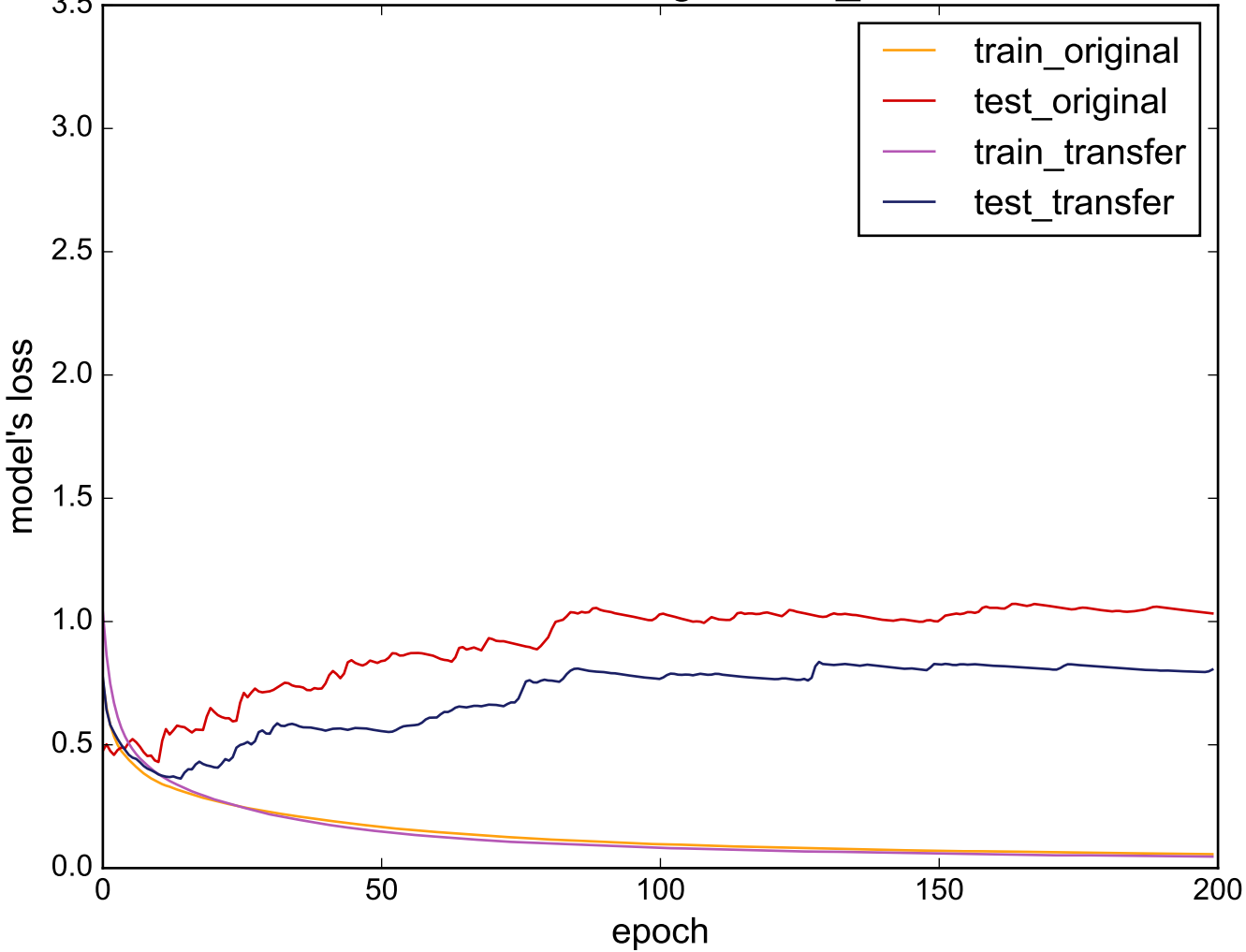
Source: wafer - Target: Two_Patterns
