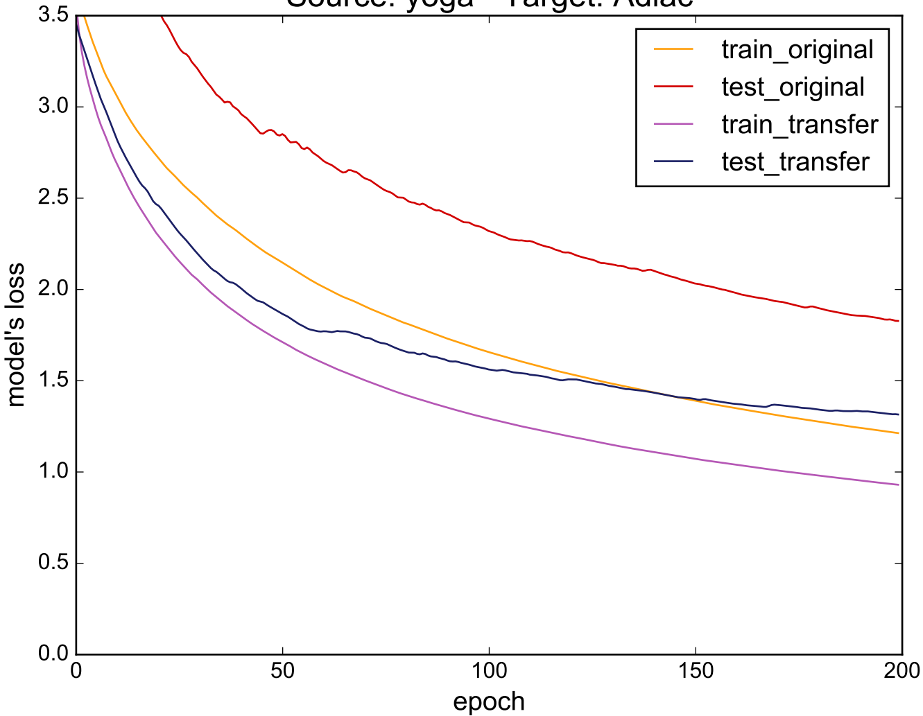
Source: yoga - Target: Adiac
