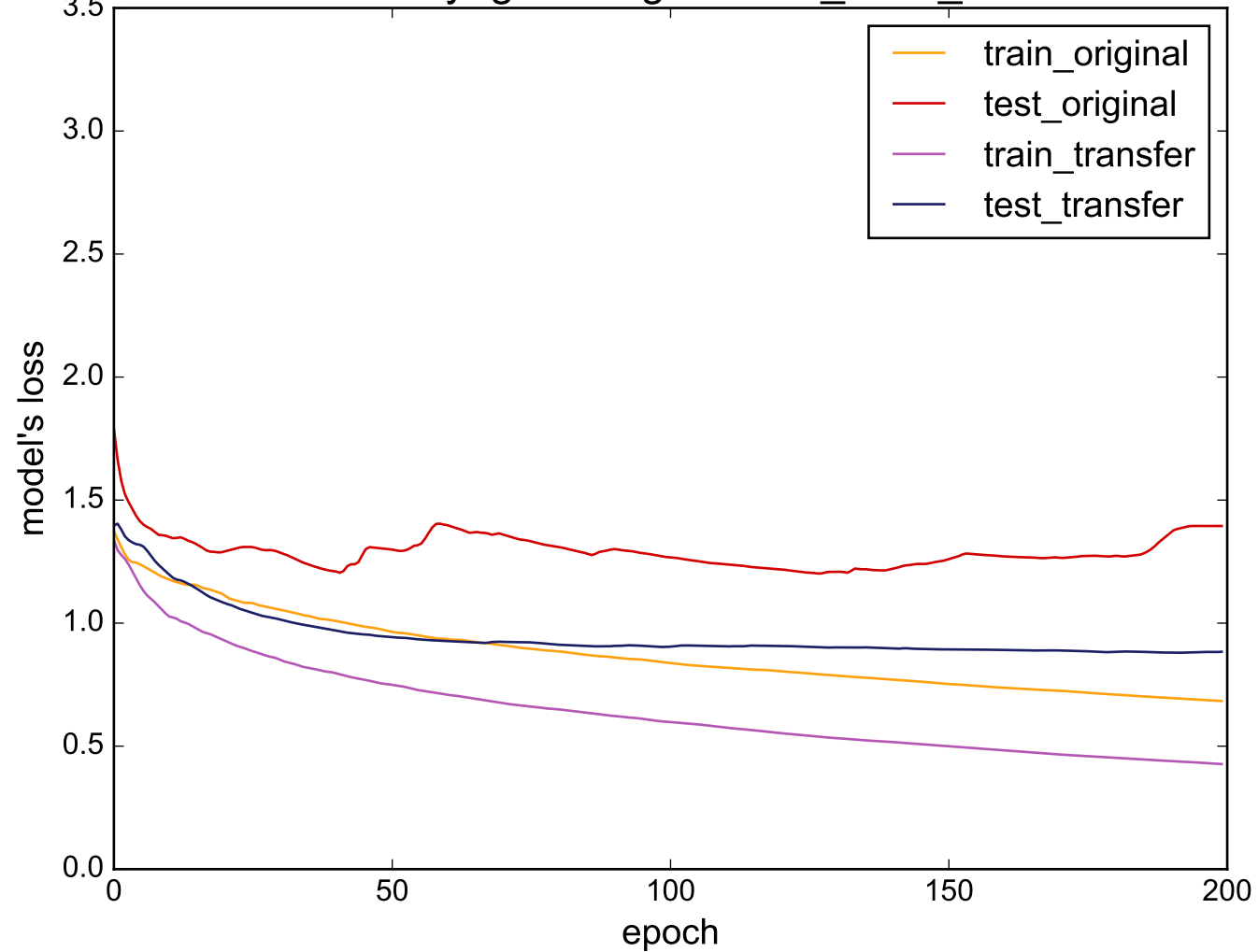
Source: yoga - Target: CinC_ECG_torso
