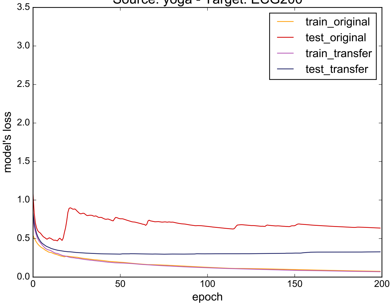
Source: yoga - Target: ECG200
