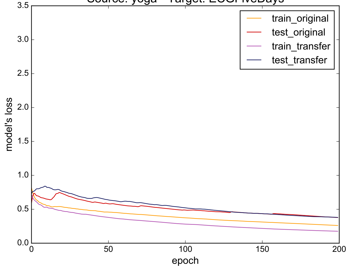
Source: yoga - Target: ECGFiveDays
