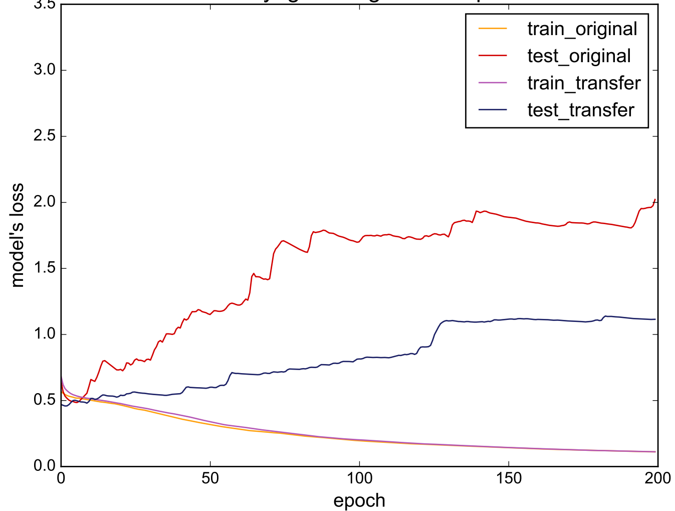
Source: yoga - Target: Earthquakes
