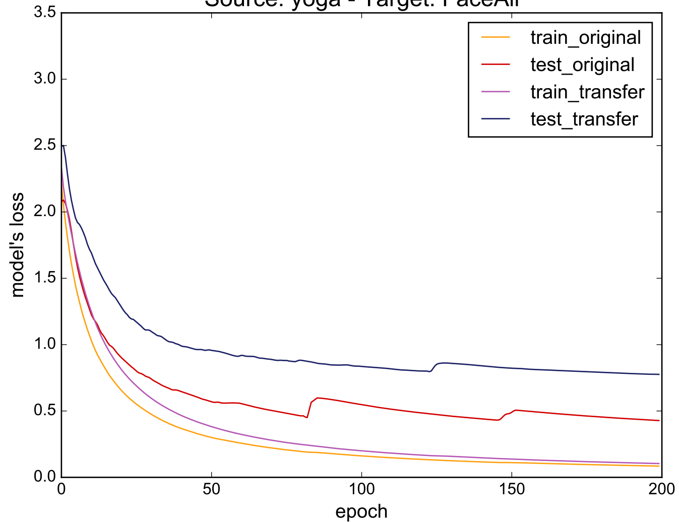
Source: yoga - Target: FaceAll
