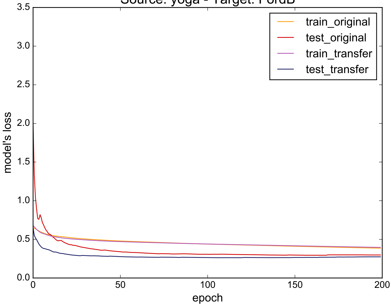
Source: yoga - Target: FordB
