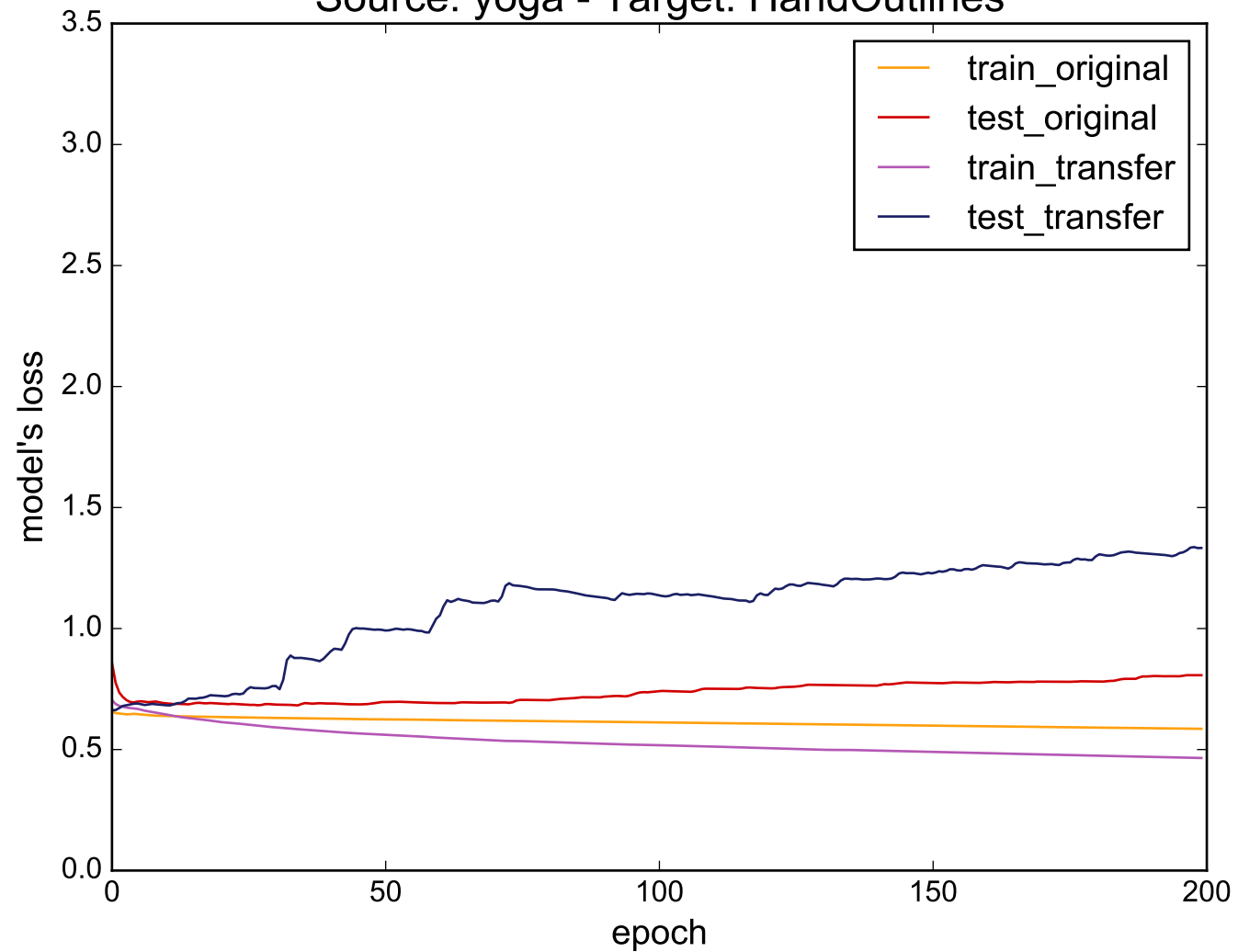
Source: yoga - Target: HandOutlines
