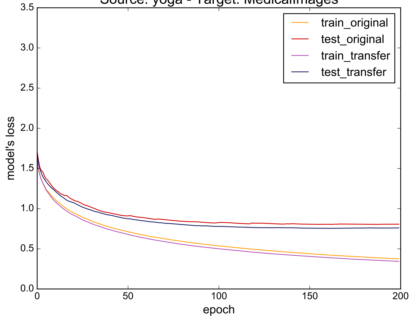
Source: yoga - Target: MedicalImages
