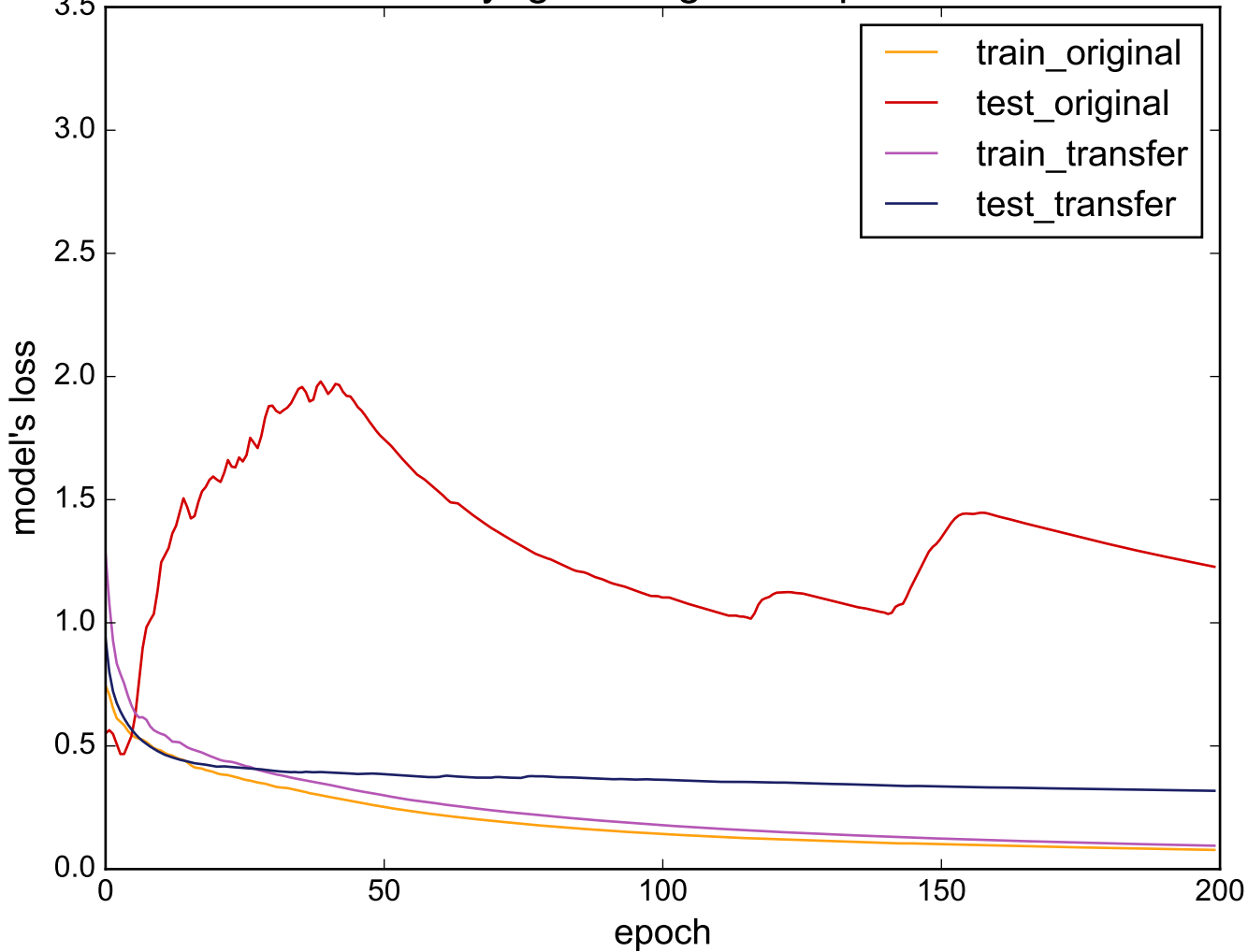
Source: yoga - Target: ShapeletSim
