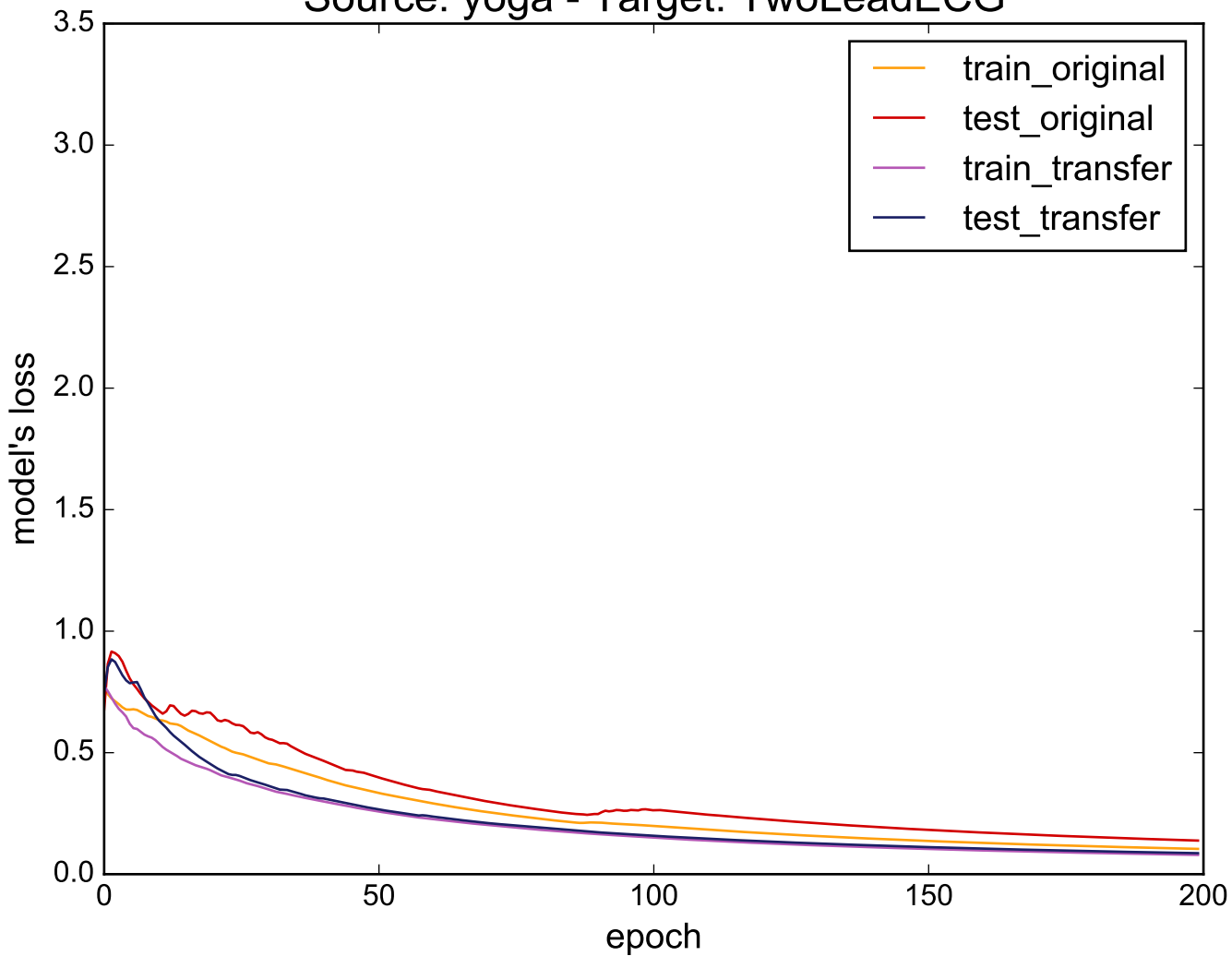
Source: yoga - Target: TwoLeadECG
